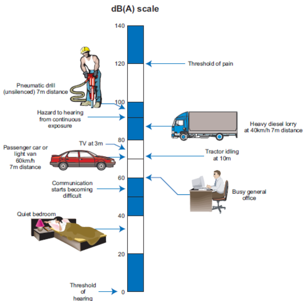
Figure 1 Typical Common Sounds on the dB (A) Scale; Source Guidelines for the treatment of Noise and Vibration in National Road Schemes, Revision 1
